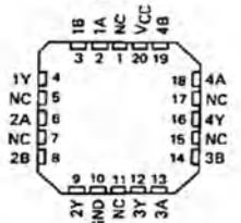
SN54LS32, SN54S32 . . . FK PACKAGE (TOP VIEW)
