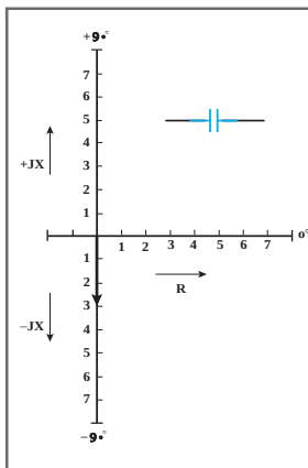
A coil with complex impedance +j\ell \Omega
